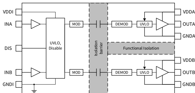
Figure 0.2 NSI6622V Block Diagram
