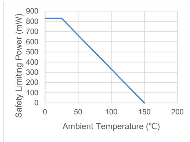
Figure 7.3 NSI66x2x-Q1SPxR Thermal Derating Curve, Dependence of Safety Limiting Values with Case Temperature per DIN VDE V 0884-17.
