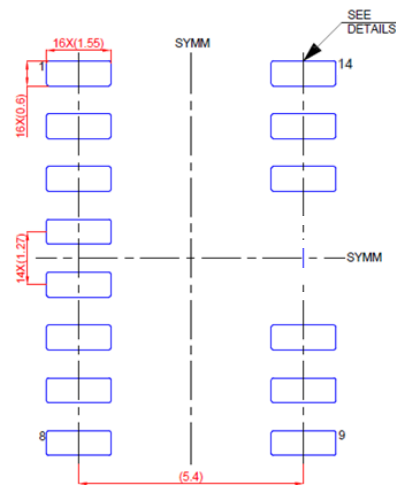
Figure 10.6 SOP14 Package Board Layout Example(mm)
