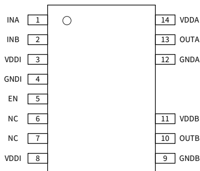
Figure 1.5 NSI6622N SOW14/ SOP14 Package
