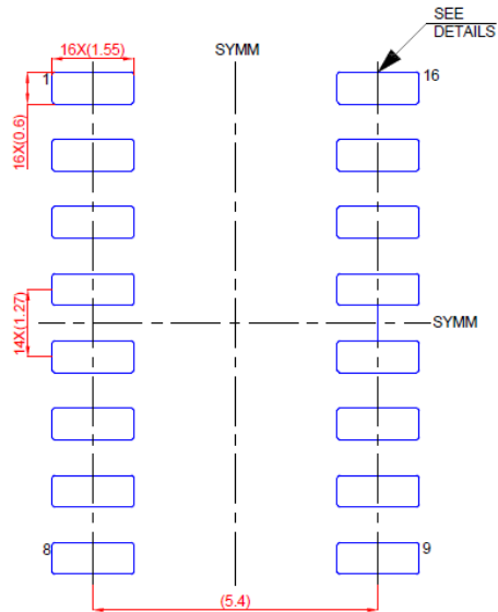
Figure 10.8 SOP16 Package Board Layout Example(mm)
